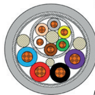
Figure 1: stepper motor harness 31.02.087-L
