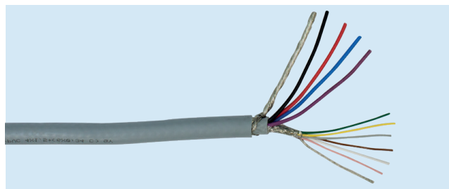
Figure 1: stepper motor harness 31.02.087-L
