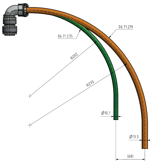
Figure 2: Reduction of bending radius old version to new version
